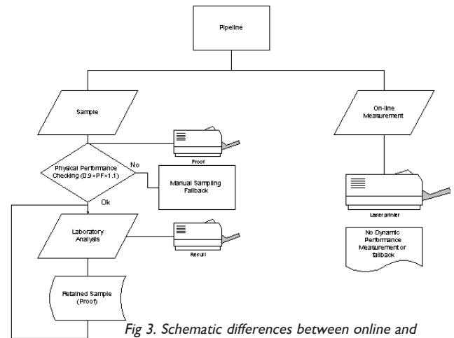
Fig 3. Schematic differences between online and sampled measurement systems
