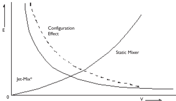
Figure 7. Energy added per Unit Volume vs. Line Velocity
