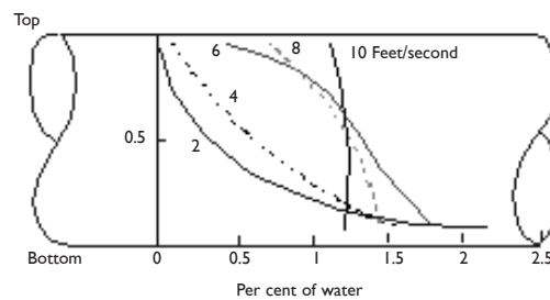
Figure 6. Concentration vs. Velocity in Horizontal Pipes
