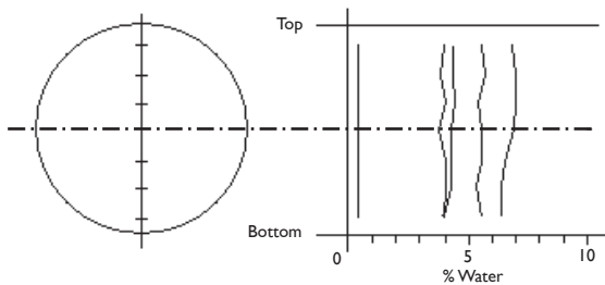
Figure 9. Multipoint Profile of a Jet Mixer on a 34" Line
