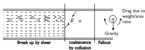
Figure 2. Droplet Break-up and Coalescence
