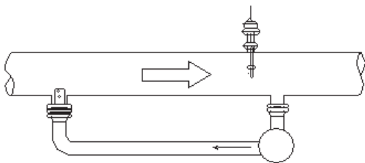
Figure 4. Jet-Mix® System
