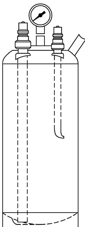
PR-53 sample receiver showing mixing internals. Mixing power is provided by Jiskoot Laboratory Mixer
